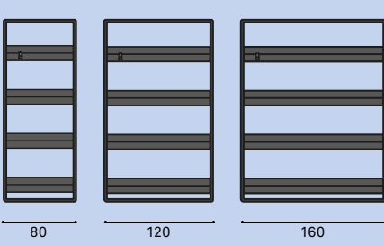
shelves - d = 25 cm (4 pieces) / Ablagen - t = 25 cm (4 Stück)
